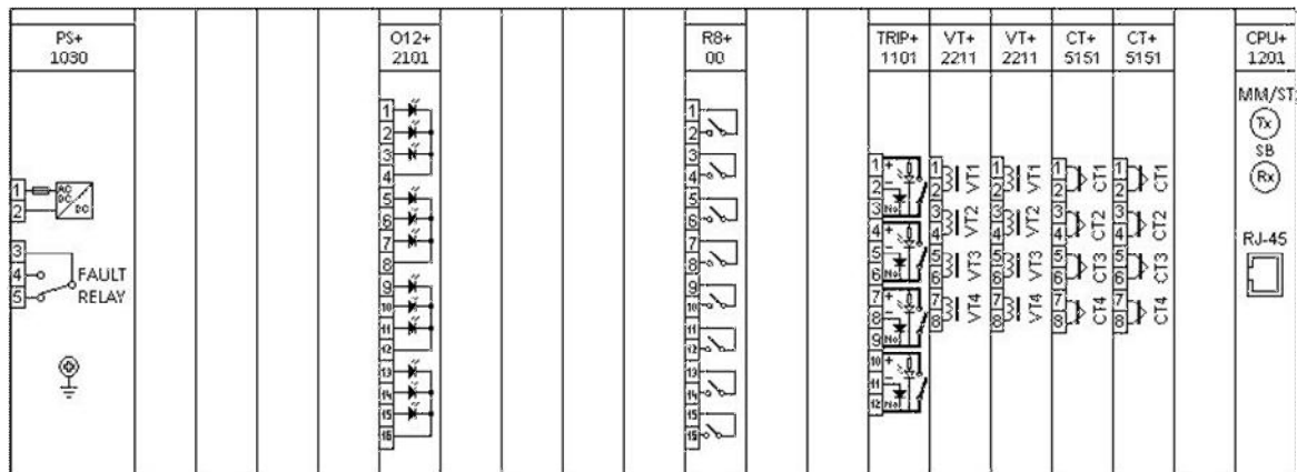
Figure 1 - Module arrangement of the DTRV-E9 configuration (rear view)
